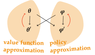
Figure 12.2: Illustration of one iteration of actor-critic methods. The dependencies between the actors and critics are shown as arrows. Methods differ in the exact order in which actor and critic are updated.
