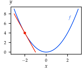
Figure A.6: The first-order characterization characterizes convexity in terms of affine lower bounds. Shown is an affine lower bound based at x = -2 .
