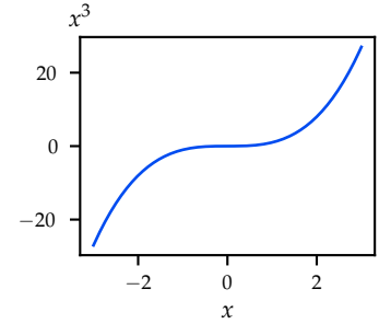
Figure A.4: Example of a saddle point at \mathbf{x} = 0 .
