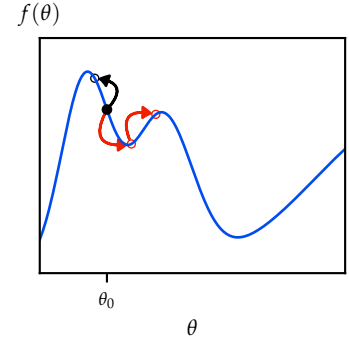
Figure 6.4: Metropolis-Hastings and Langevin dynamics minimize the energy function f(\theta) shown in blue. Suppose we start at the black dot \theta_0 , then the black and red arrows denote possible subsequent samples. Metropolis-Hastings uses an “uninformed” search direction, whereas Langevin dynamics uses the gradient of f(\theta) to make “more promising” proposals. The random proposals help get past local optima.
