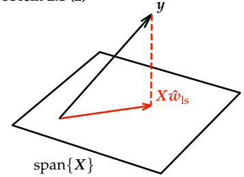
Figure 2.2: Least squares regression finds the orthogonal projection of \mathbf{y} onto \text{span}\{\mathbf{X}\} (here illustrated as the plane).
